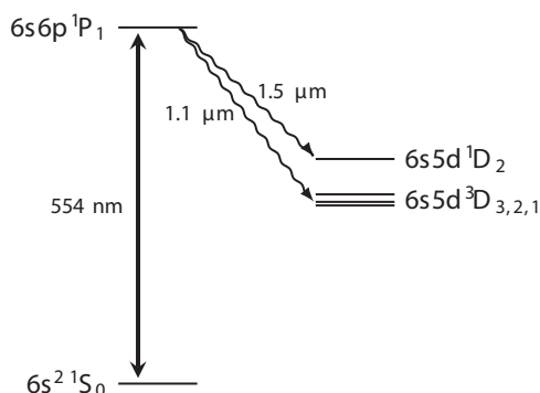
Fig. 10. Energy-level diagram of the neutral barium atom, showing the levels and transitions involved in the experiment of Finn and Greenlees.
