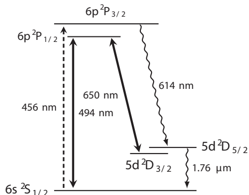
Fig. 8. Energy-level diagram of Ba^+ , showing the levels and transitions involved in the experiments of the University of Washington and University of Hamburg groups.
