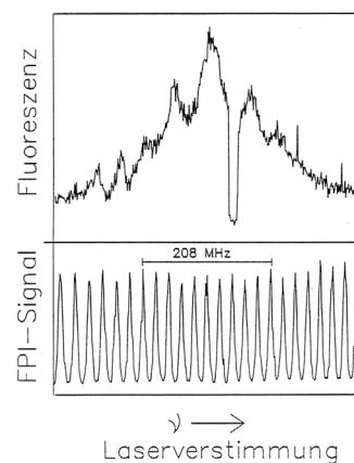
Fig. 9. Early data (1984–1985) from the University of Hamburg group [13, Fig. 28]. Resonance fluorescence of a single Ba^+ ion as a function of the frequency of the 650 nm laser (top). Transmission signal of Fabry-Pérot interferometer used for frequency calibration (bottom). The laser frequency and time increase from left to right. The sudden decrease in fluorescence followed by a sudden increase is probably due to quantum jumps to and from the 5d^2D_{5/2} dark state. The multiple peaks in the signal are probably due to rf micromotion of the ion. (Number of data points = 370, time per point = 1 s.)
