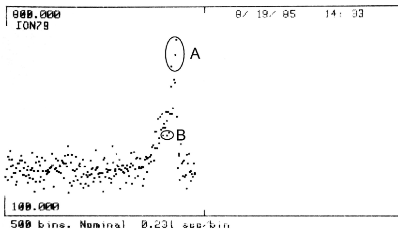
Fig. 4. Fluorescence detected from the 194 nm transition of an Hg + ion. The 194 nm laser frequency increases from left to right. Dots within the ellipses marked A and B represent periods when the ion spent the least or most time, respectively, in a metastable state. The vertical scale is in frequency units (counts per second). The number of photons counted is given by the number of counts per second multiplied by the time bin (0.231 s). This number can be used to estimate the statistical noise of photodetection. The vertical scale limits are 2.31 and 184.8 counts per bin. The background can be estimated from the low-laser-frequency data.
