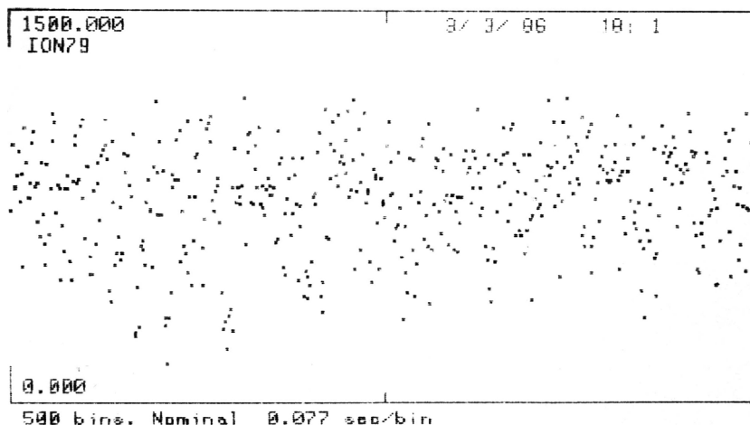
Fig. 5. Sequence of 194 nm Hg + fluorescence measurements of duration 77 ms. Vertical scale limits are 0 and 11.55 counts per bin. Frequency of laser is fixed and close to resonance. Measurement time increases from left to right. The lowest-fluorescence measurements represent periods when the ion spent much of the time in a metastable state. No background has been subtracted from the data.
