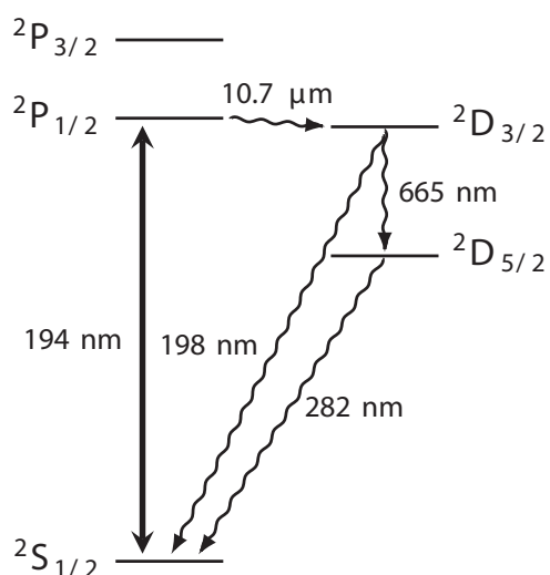
Fig. 3. Energy-level diagram of the Hg + ion and radiative decays relevant to the NIST experiment with only the 194 nm laser applied.
