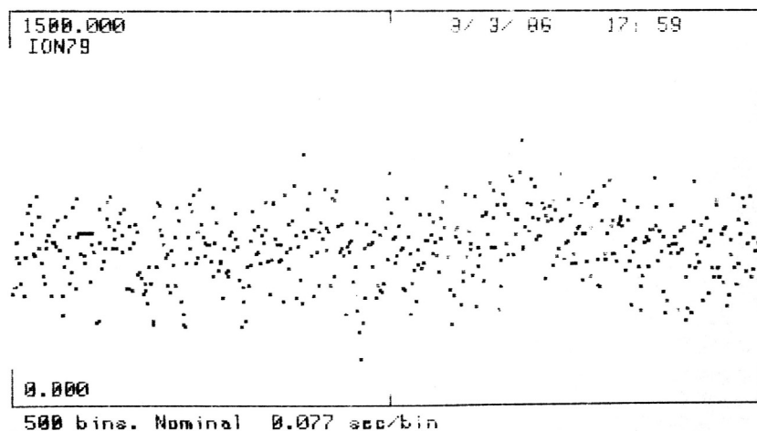
Fig. 6. Sequence of 194 nm Hg + fluorescence photocounts of duration 77 ms. Frequency of laser is fixed and detuned further below resonance, compared to Fig. 5. The horizontal and vertical scales are the same as in Fig. 5.
